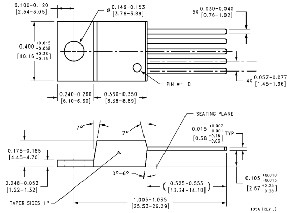
5-Lead Molded TO-220 (T) Order Number LM2941CT NS Package Number T05A
